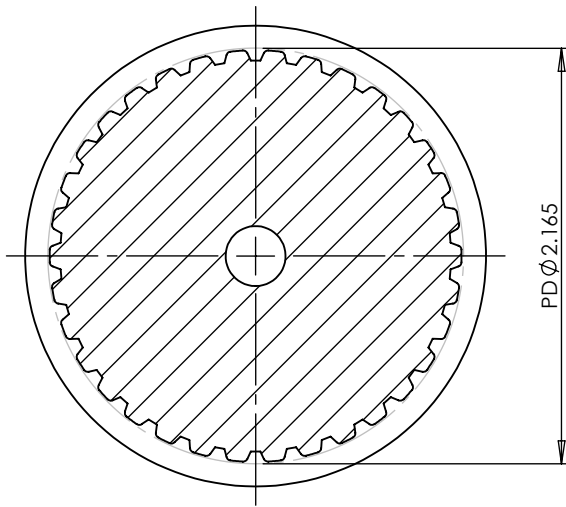
SECTION B-B
